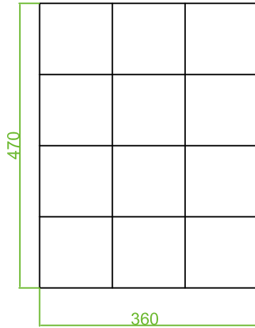
吸塑 Blister-A(B)-470*360*25
